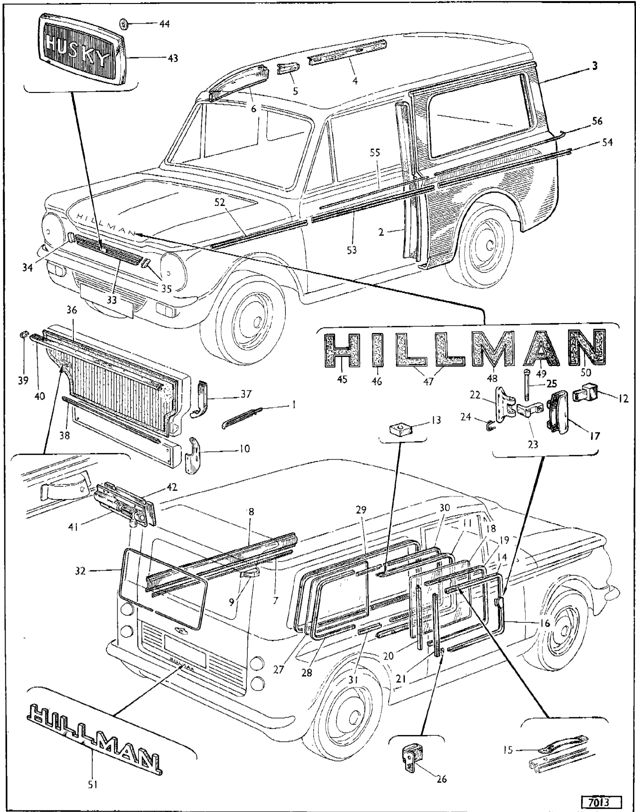
SECTION QB
