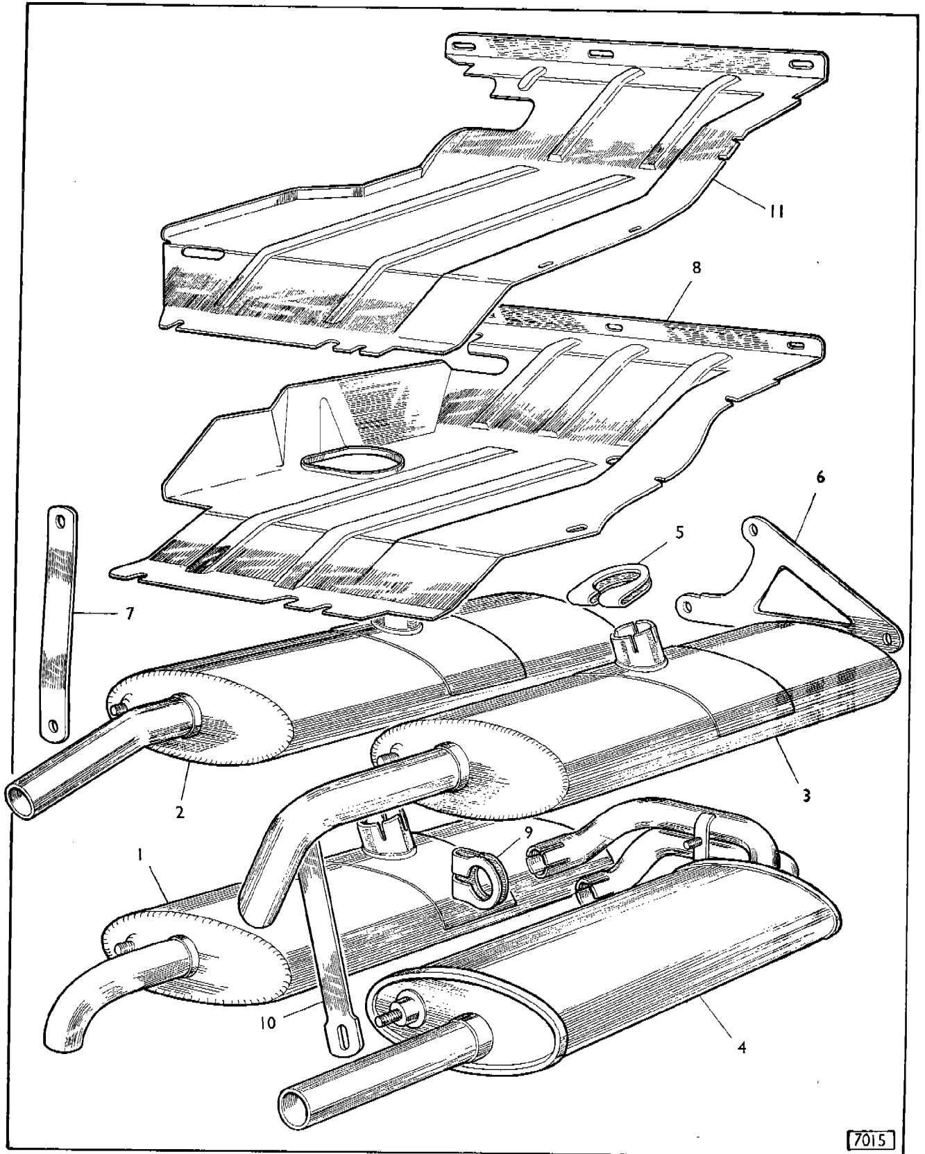
SECTION N
